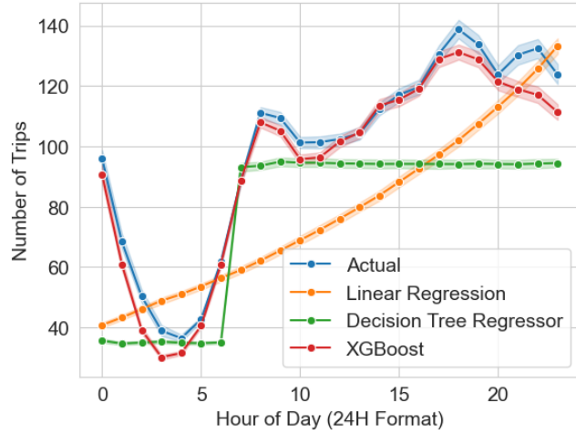
Figure 7: Errors on Test Data by Hour
